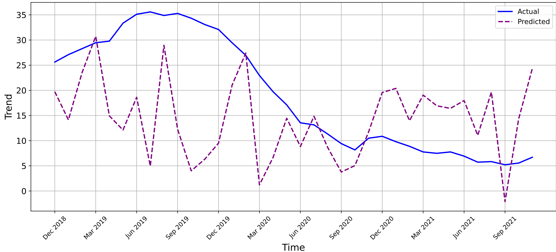
Solution_BLACKHOLING_Mentions - Validation
